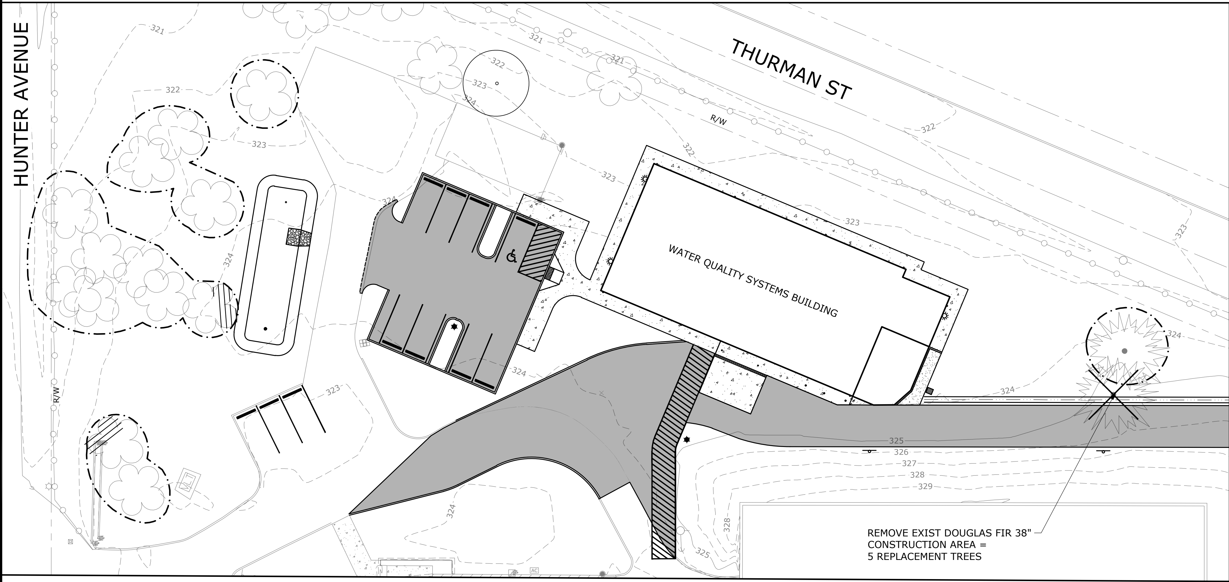
WATER QUALITY SYSTEMS BUILDING AREA SCALE: 1"=20'
